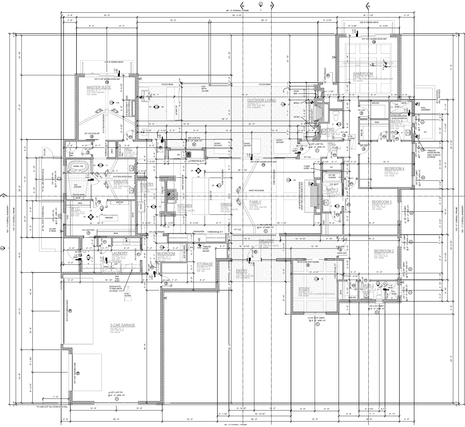
1 FIRST FLOOR 1/4" = 1'-0"
